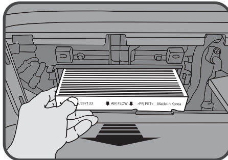
6. Ensure the airflow arrow points downward, then reinstall all components in the reverse order of disassembly.
