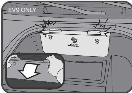
3. Carefully pull the tabs forward to detach the HVAC access cover.
